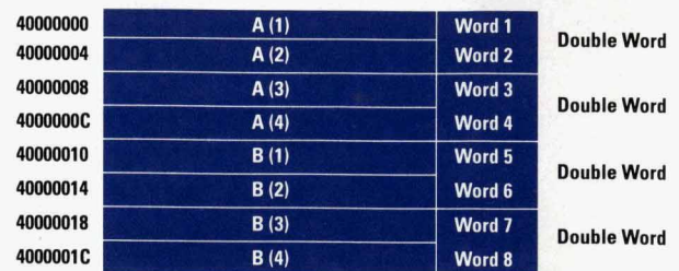
Fig. 1. The arrangement of vectors A and B in memory. All the elements are double-word-aligned.
