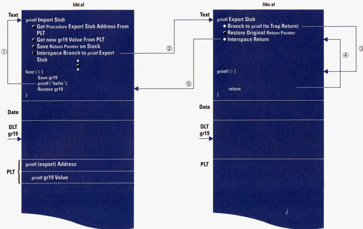
Fig. 7. Shared library procedure calls.
