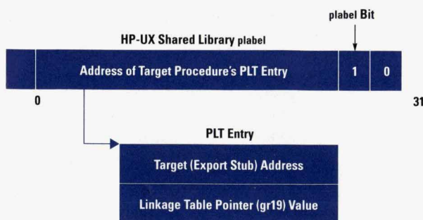
Fig. 6. A shared library label and PLT entry.
