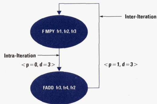
Fig. 6. A dependency graph.
