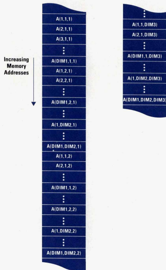
Fig. 1. Column-major storage layout for array A.
