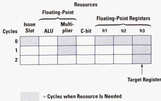
Fig. 5. An example of a resource reservation table for the FMPY instruction.
