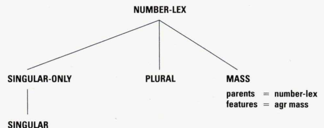
Fig. 6. An excerpt from the word class hierarchy for the word class Mass.
