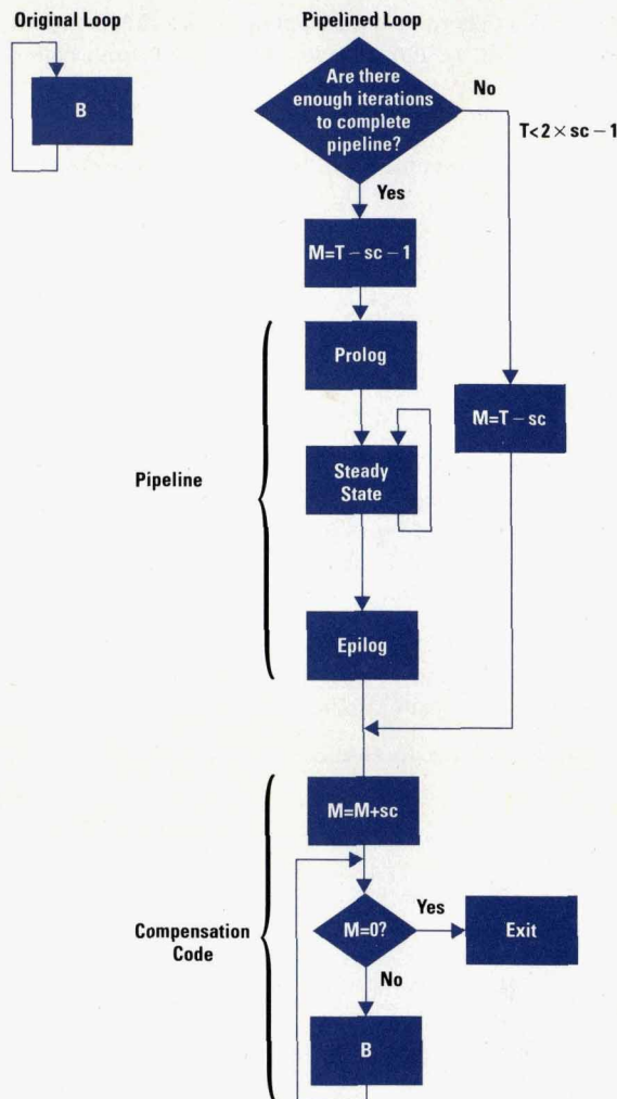
Fig. 9. Loop transformation to add compensation code to make sure the pipelined loop executes the same number of times as the original loop. Block B represents the original loop and the case in which the loop does not execute enough times to reach the pipeline.
